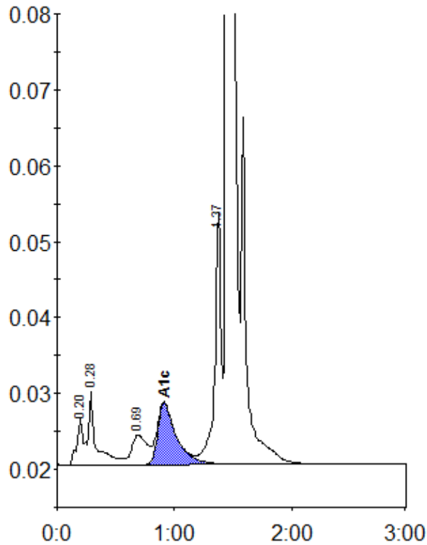
Peak table - ID: 10315331
