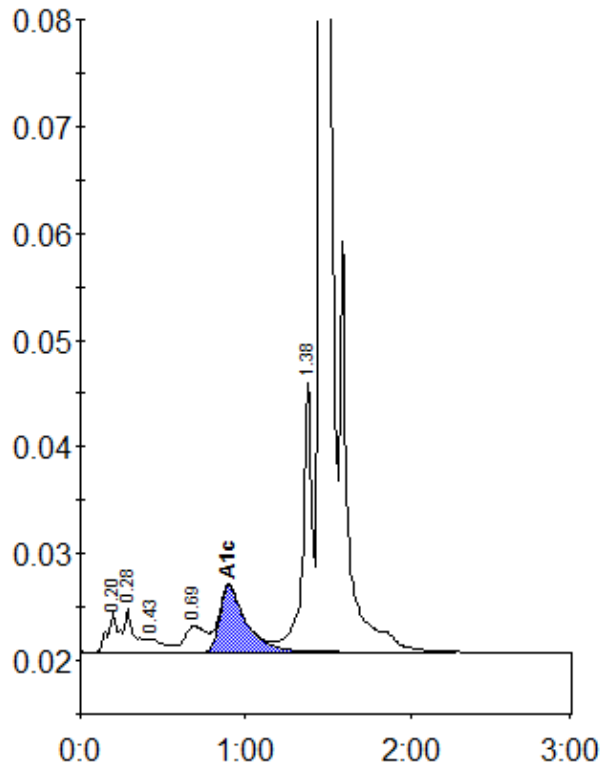
Peak table - ID: 10259250
