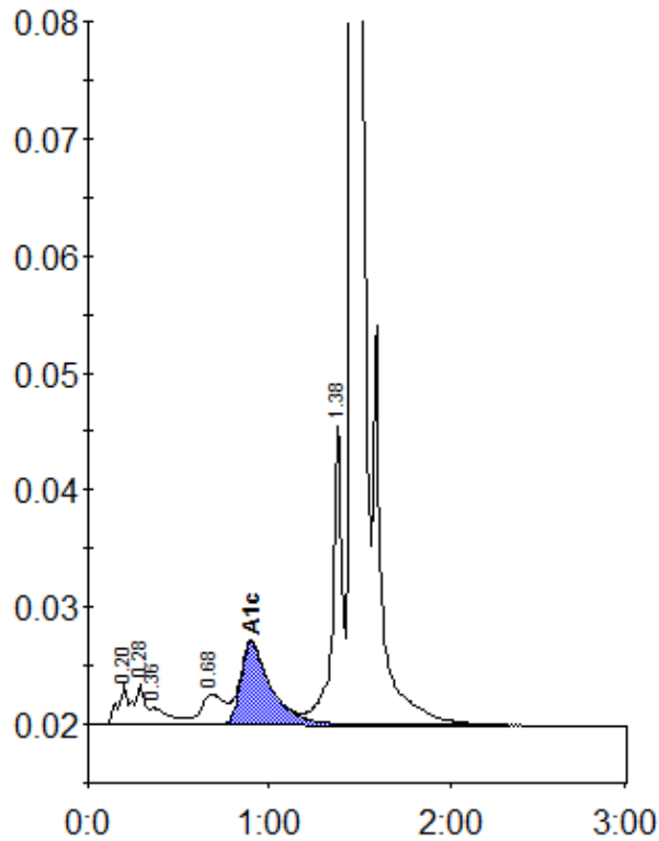
Peak table - ID: 10340454
