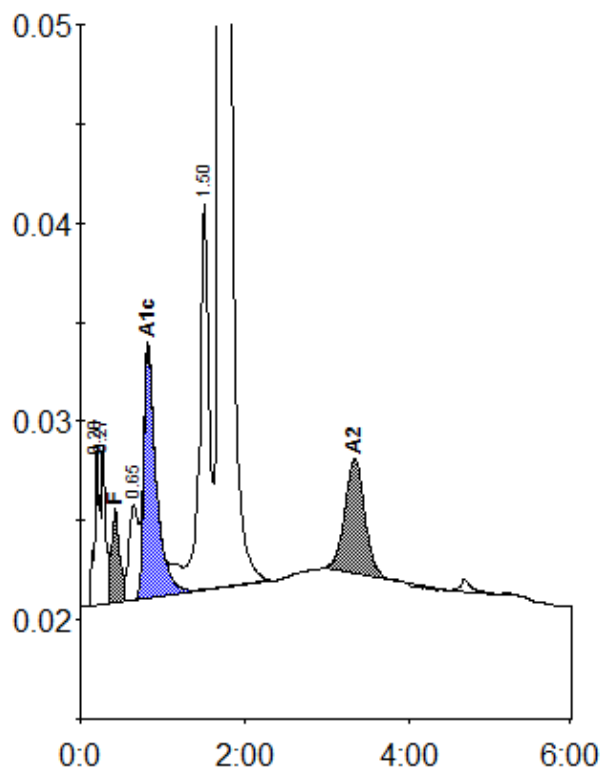
Peak table - ID: 10366487
