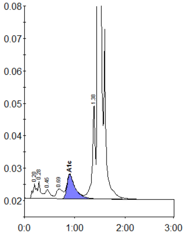
Peak table - ID: 10373890
