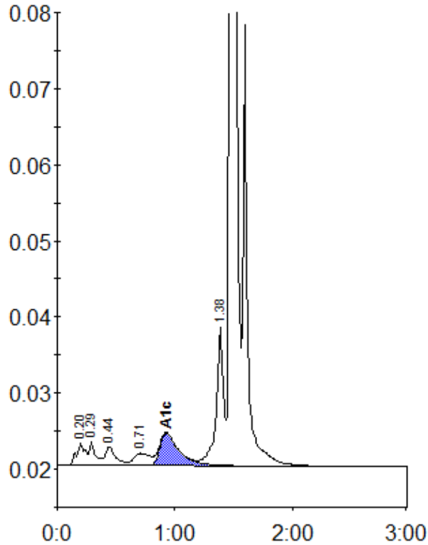
Peak table - ID: 10340835
