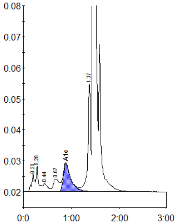
Peak table - ID: 10251677
