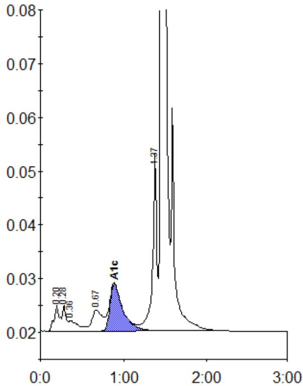
Peak table - ID: 10251672
