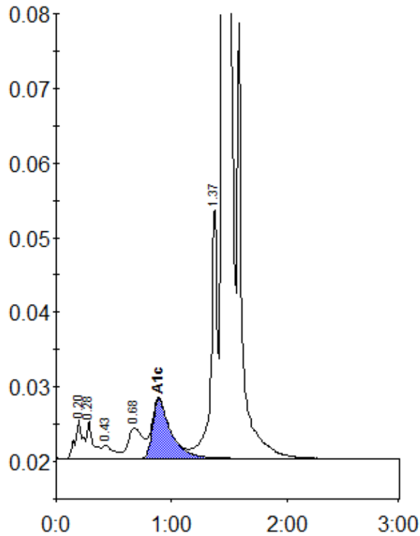
Peak table - ID: 10392584
