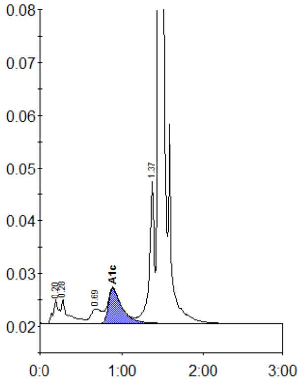
Peak table - ID: 10374738
