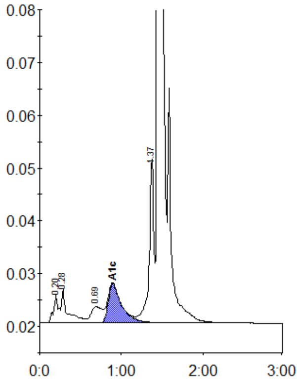
Peak table - ID: 10374711
