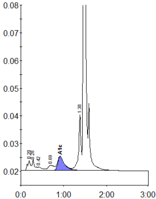
Peak table - ID: 10290165
