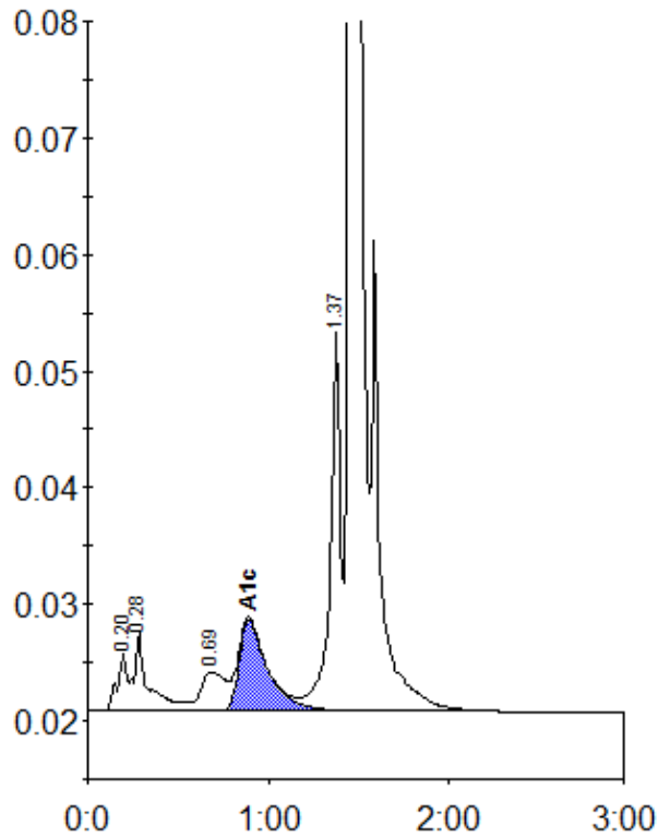
Peak table - ID: 10402492
