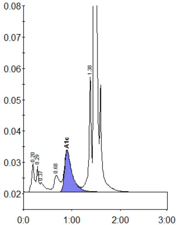
Peak table - ID: 10051317
