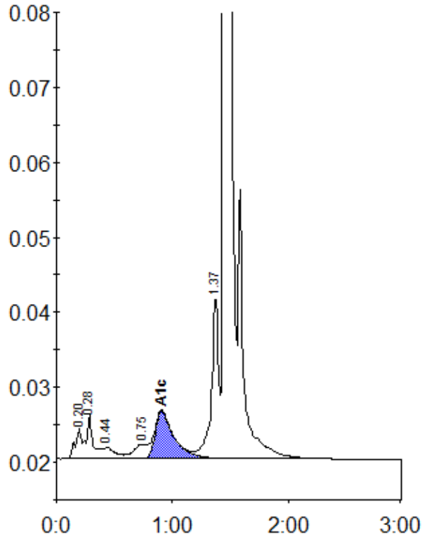
Peak table - ID: 10370960
