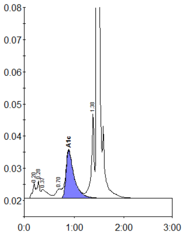
Peak table - ID: 10318607
