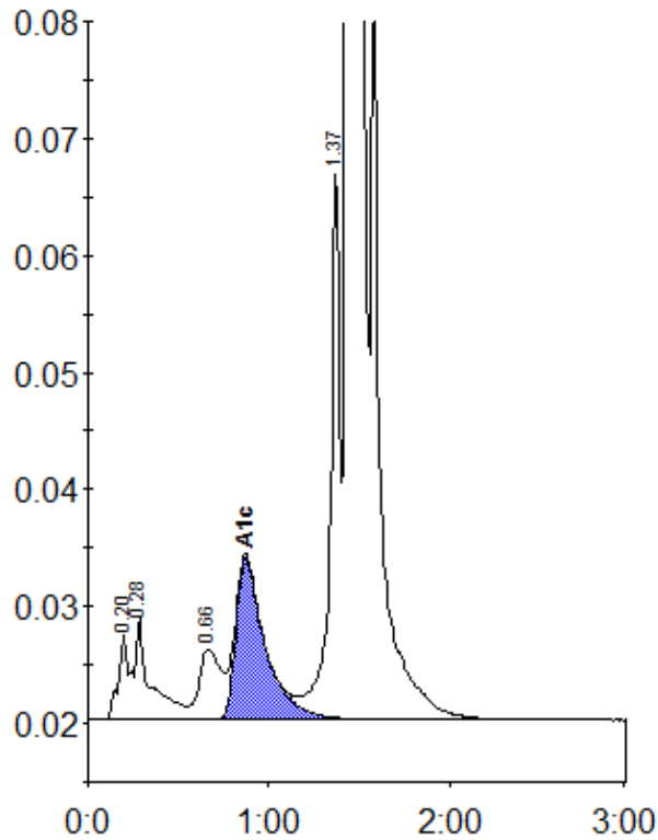
Peak table - ID: 10402861
