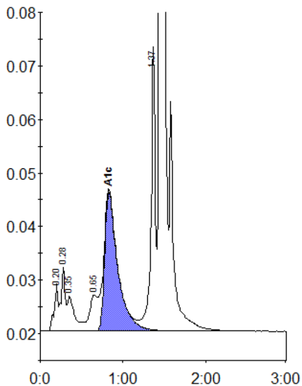
Peak table - ID: 10261452
