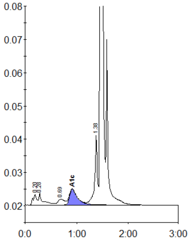
Peak table - ID: 10363609
