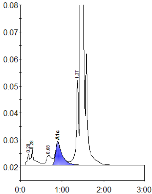
Peak table - ID: 10189173
