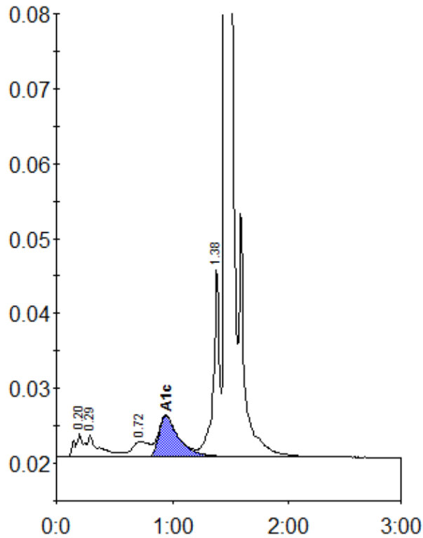
Peak table - ID: 10258622
