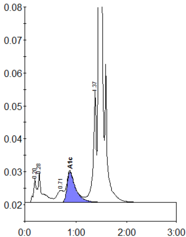
Peak table - ID: 10316710
