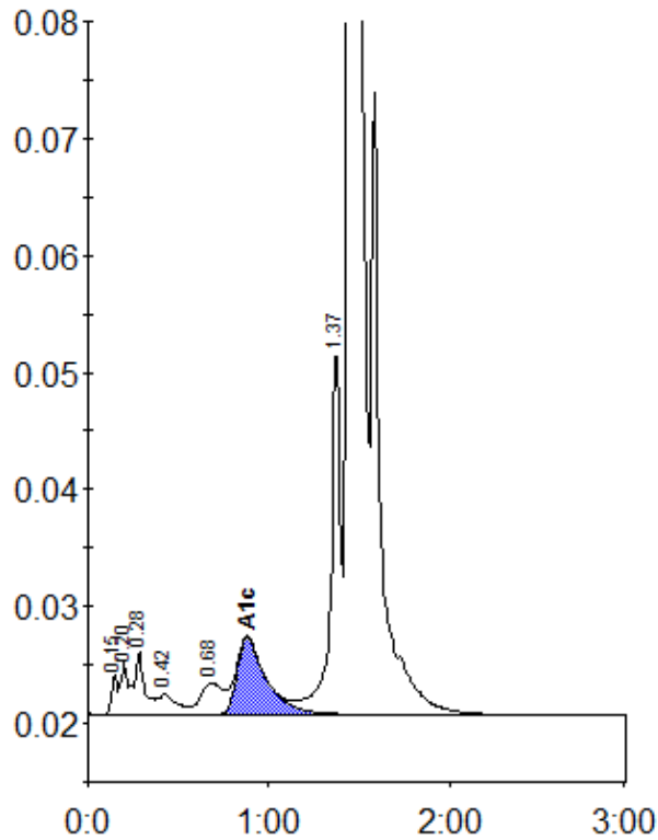
Peak table - ID: 10268555
