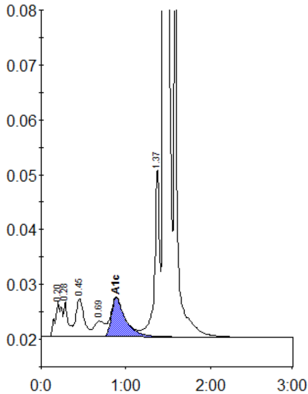
Peak table - ID: 10272080
