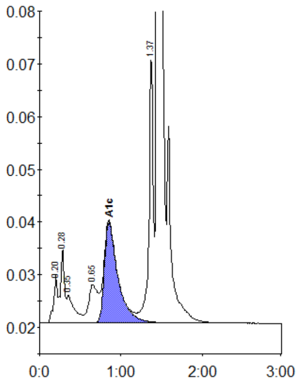
Peak table - ID: 10245351
