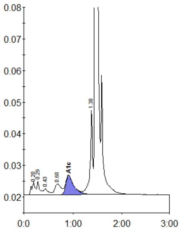
Peak table - ID: 10246442
