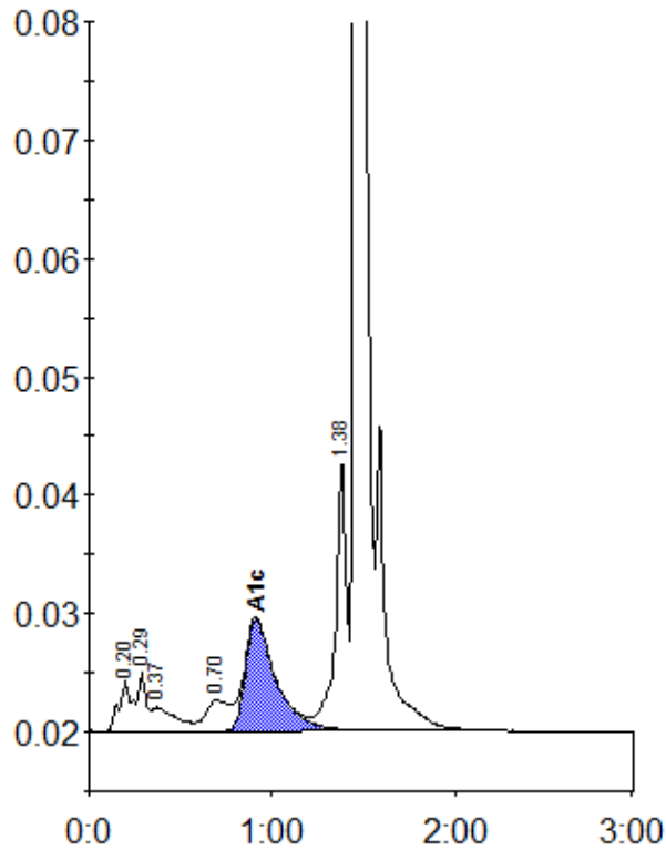
Peak table - ID: 10245740
