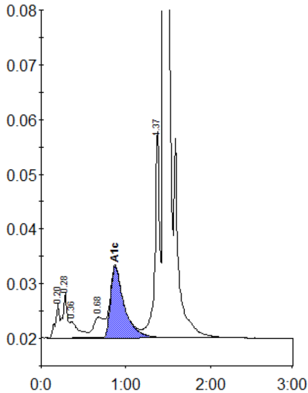
Peak table - ID: 10258356
