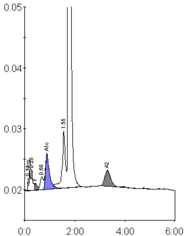
Peak table - ID: 10227036
