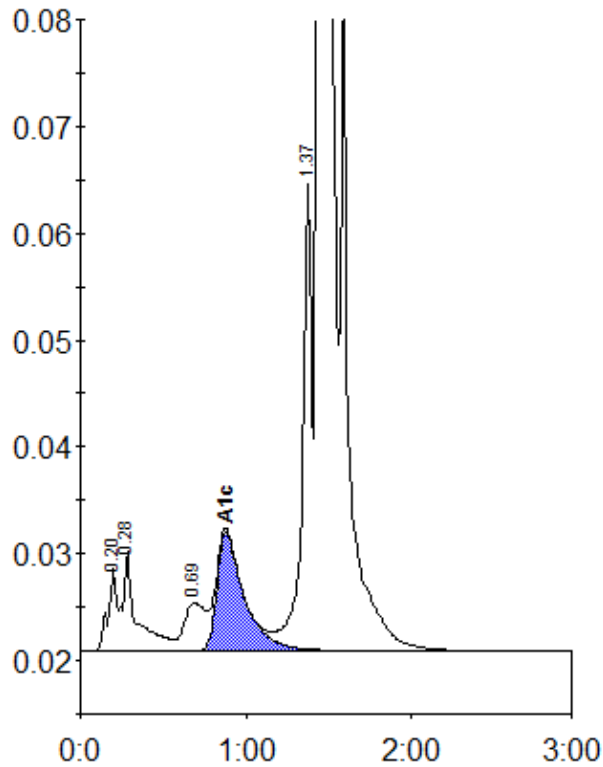
Peak table - ID: 10285361
