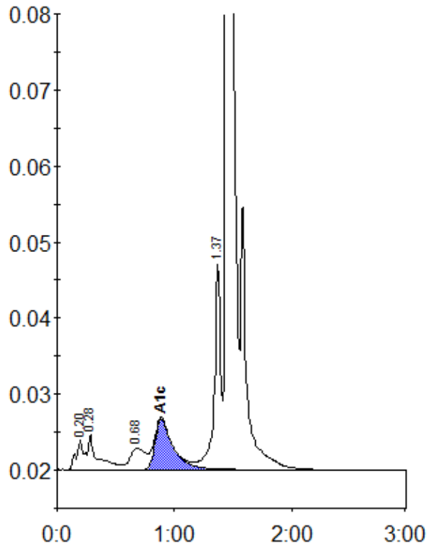
Peak table - ID: 10266130
