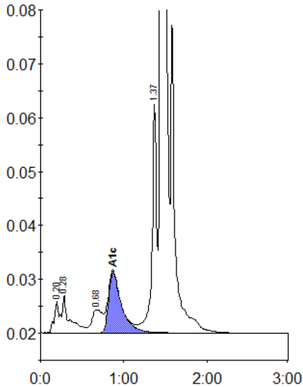
Peak table - ID: 10297645
