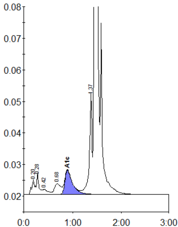
Peak table - ID: 10241506
