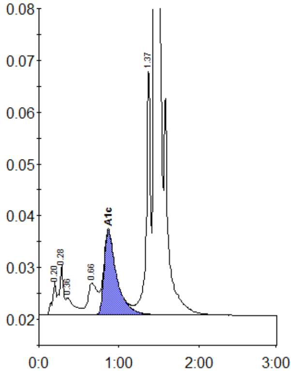
Peak table - ID: 10312243
