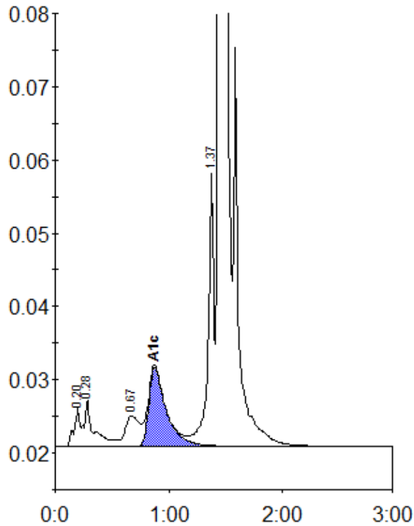
Peak table - ID: 10247888
