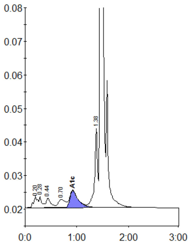
Peak table - ID: 10258937
