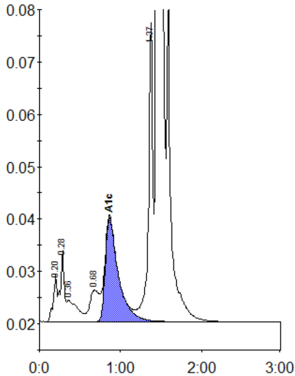
Peak table - ID: 10272525
