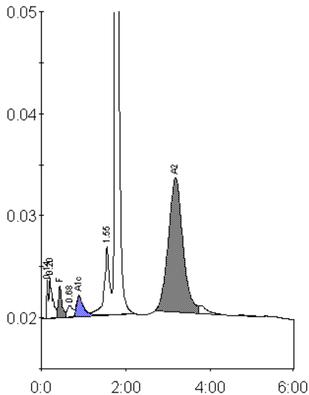
Peak table - ID: 10131041
