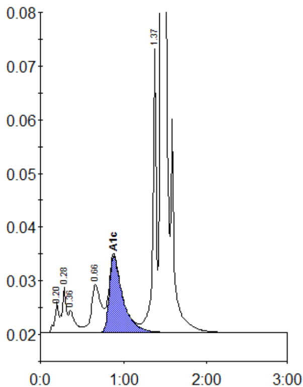
Peak table - ID: 10315023
