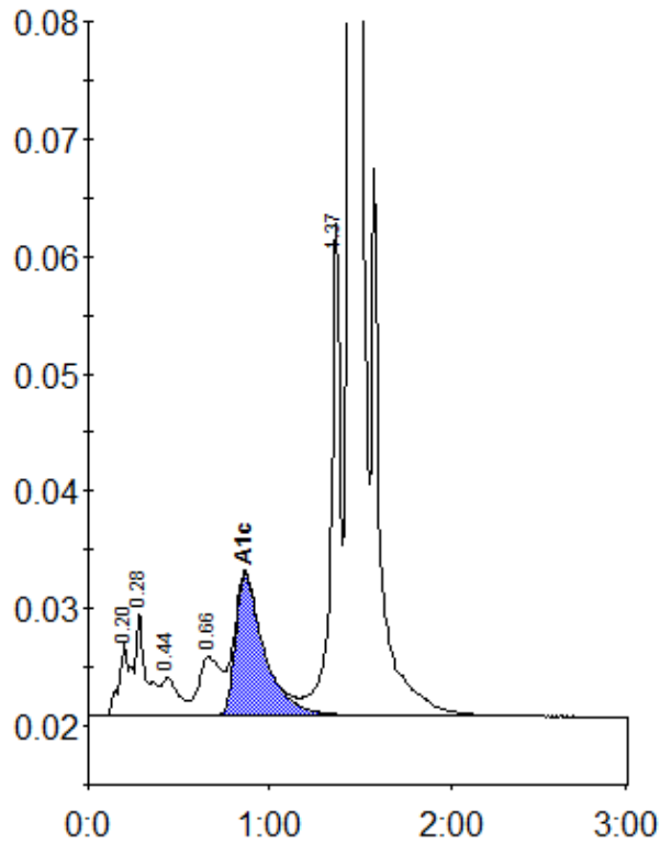
Peak table - ID: 10312444
