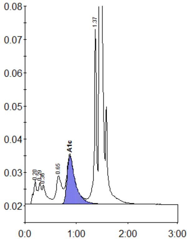
Peak table - ID: 10163007
