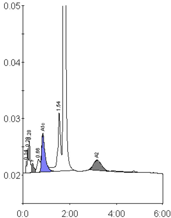
Peak table - ID: 10312662
