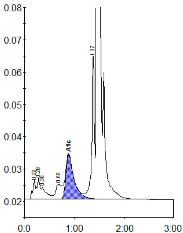
Peak table - ID: 10290644
