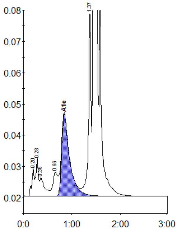
Peak table - ID: 10290649
