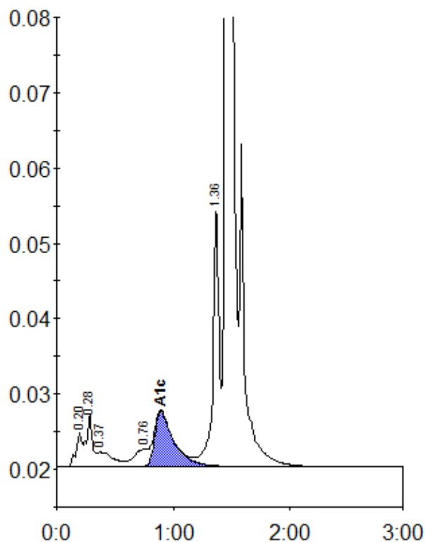
Peak table - ID: 10310227
