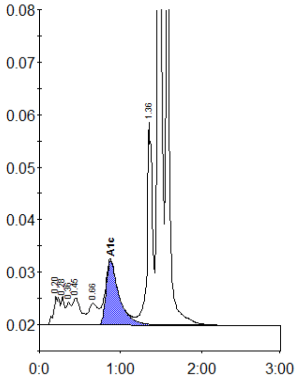
Peak table - ID: 10269249
