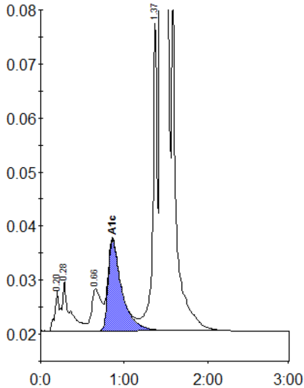
Peak table - ID: 10240283
