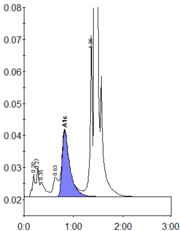
Peak table - ID: 10194053
