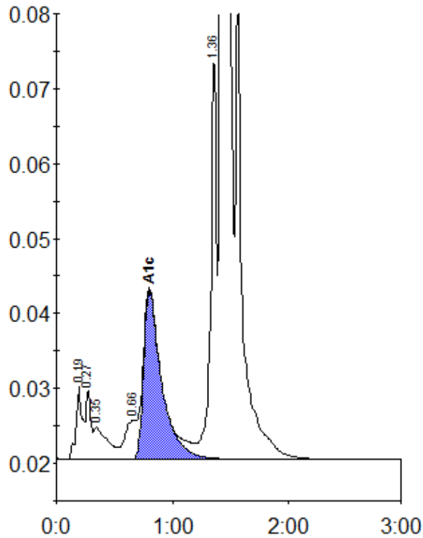
Peak table - ID: 10194611
