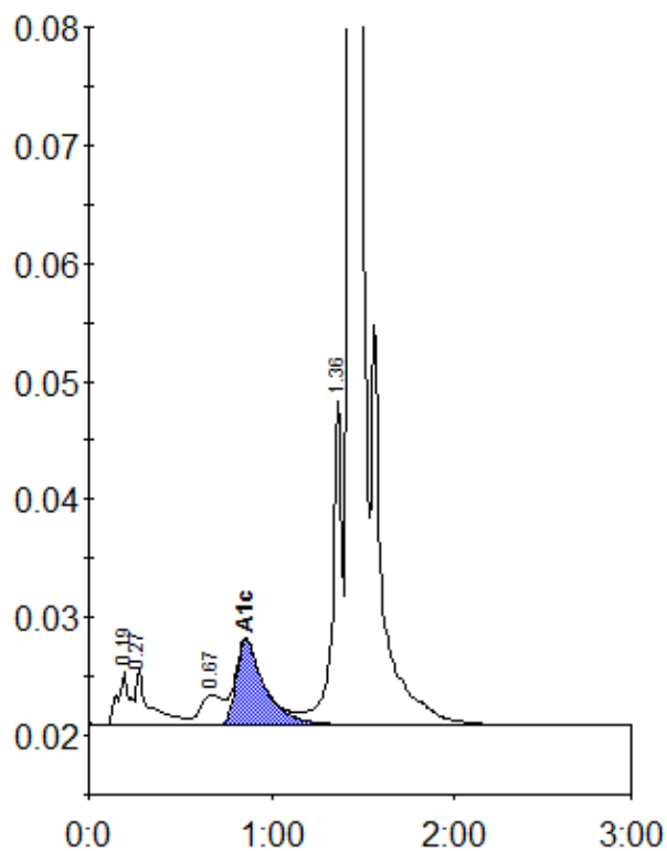
Peak table - ID: 10316750
